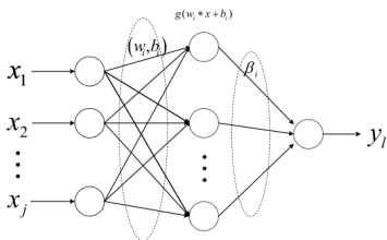
Topology of the NNA Artificial Neuron
